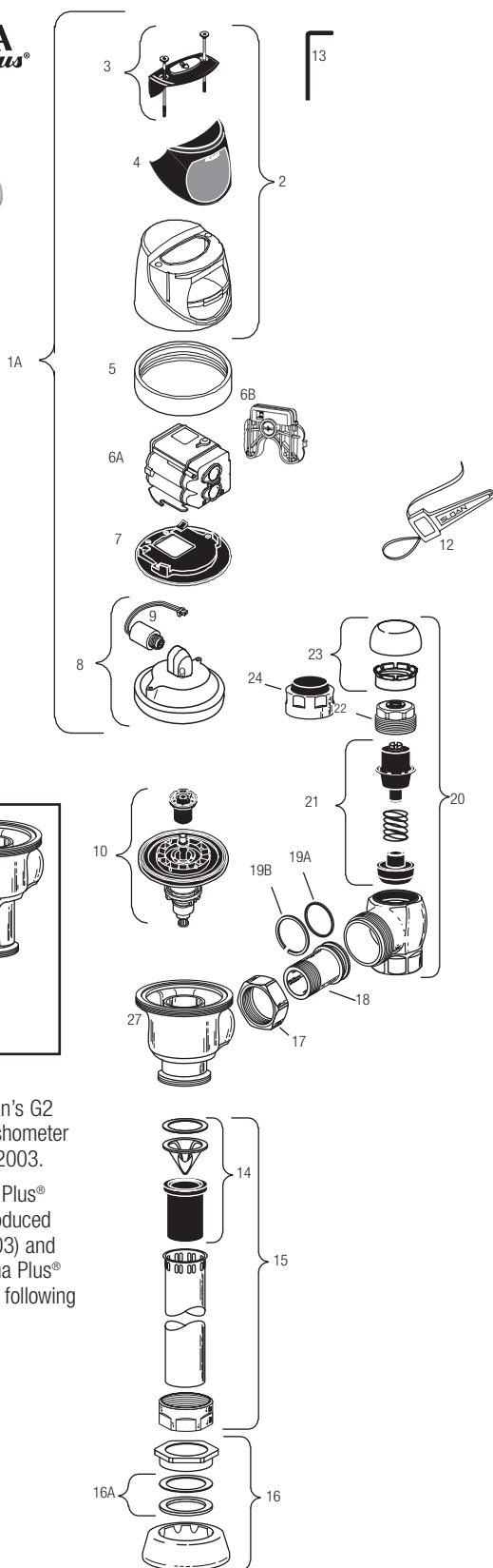
EARLIER MODEL WITH A-3 BODY
