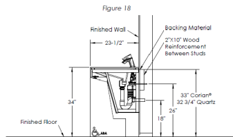
Rough-In (Three Station): Section View
