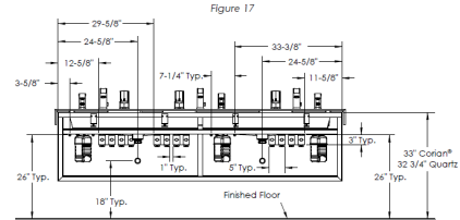
Rough-In (Three Station): Plumbing and Electrical, Front View
