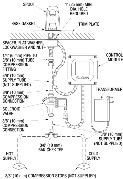
ETF-610 Faucet with Bak-Chek® Tee for Hot and Cold Water Supply (shown with 4" trim plate)
