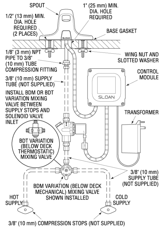
ETF-600 Faucet with BDM and BDT Variation Mixing Valves for Hot and Cold Water Supply
